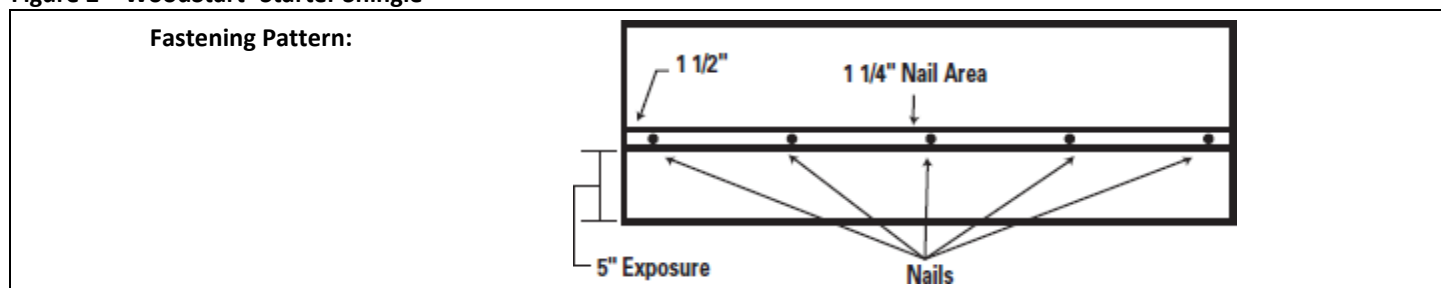
Figure 2 – WoodStart® Starter Shingle
