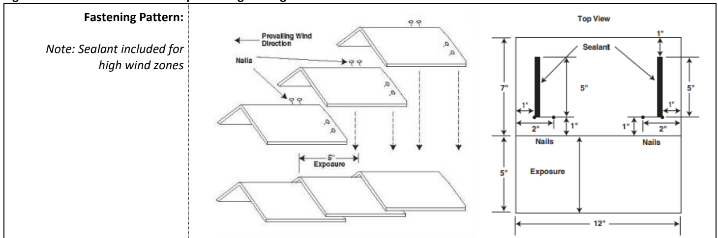
Figure 14 – WeatherGuard® HP Hip and Ridge Shingles
